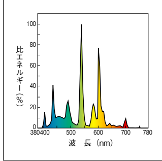
3波長形白色:EX-W(EW)
