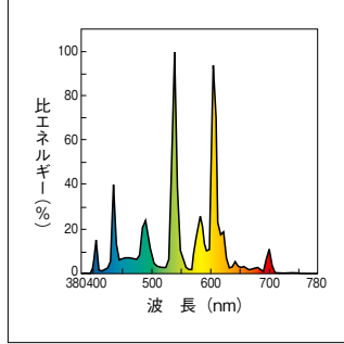
3波長形温白色:EX-WW(EWW)
